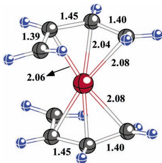
Figure 8. The ground-state geometry of cationic \text{Ni}^+(\text{C}_4\text{H}_6)_2 complex. Bond lengths are given in angstroms ( \text{\AA} ).
